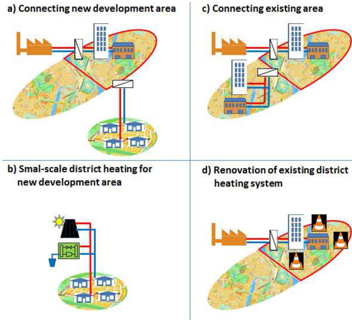
Figure 2.7: Development scenarios for low temperature district heating (Olsen, Christiansen et al. 2014).
