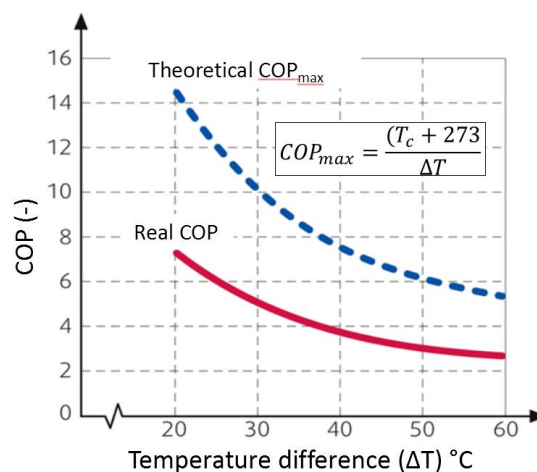
Figure 2.5: Connection between Coefficient of Performance (COP) and the temperature difference between the heat source and the heat supply ( \Delta T ) (Stene 2009)
