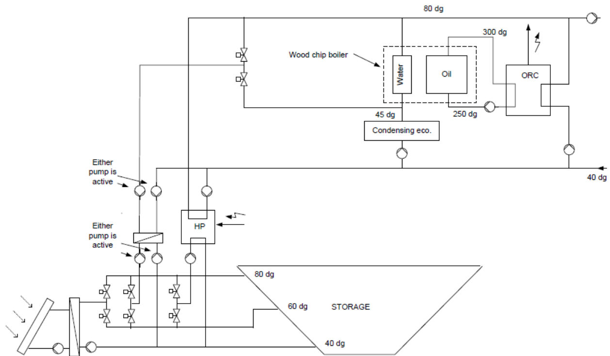
Figure 3.12: System configuration of Marstal District Heating (Jensen 2014)
