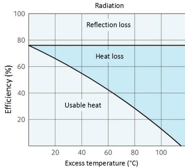
Figure 2.4: Connection between excess temperature (difference between water temperature and ambient temperature) and efficiency of solar collectors (Simonsen 2011).
